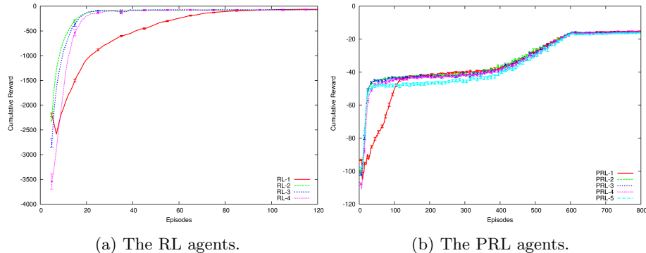
Figure 7: Reward accumulated by the learning agents with different knowledge representations
