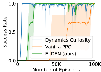
(b) ELDEN performs worse than Dynamics Curiosity
