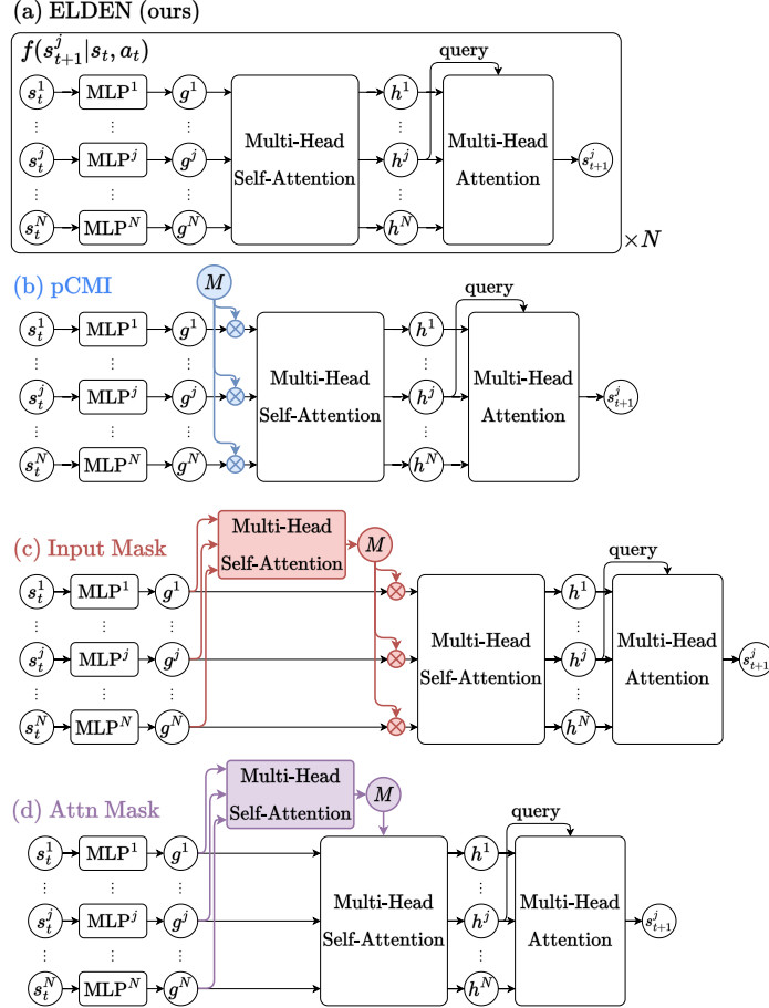
Figure 5: The dynamics model of each local dependency detection method. (a) The dynamics model of ELDEN for predicting s_{t+1}^j . Notice that each network predicts s_{t+1}^j only, and there are N such networks in total, each responsible for predicting one state factor in s_{t+1} . For visual simplicity, the “ \times N ” symbol is only shown in (a). (b) pCMI computes p(s_{t+1}^j | s_t, a_t) and p(s_{t+1}^j | s_t \setminus s_t^i, a_t) by manually setting the binary mask M to different values, where \otimes represents element-wise multiplication. (c) For Input Mask, M is learned to condition on (s_t, a_t) and is regularized to use as few inputs as possible. (d) For Attn Mask, M also conditions on (s_t, a_t) but is applied to the attention score in the self-attention module.
