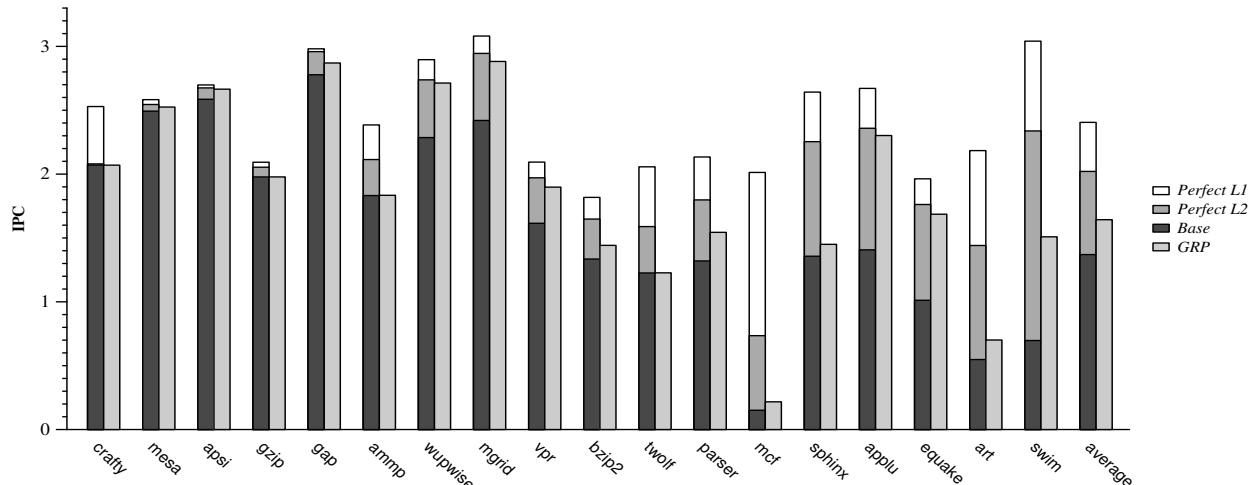
Figure 1: Processor performance
