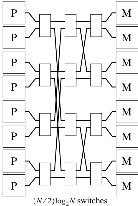
Figure 1. Dancehall architectures
