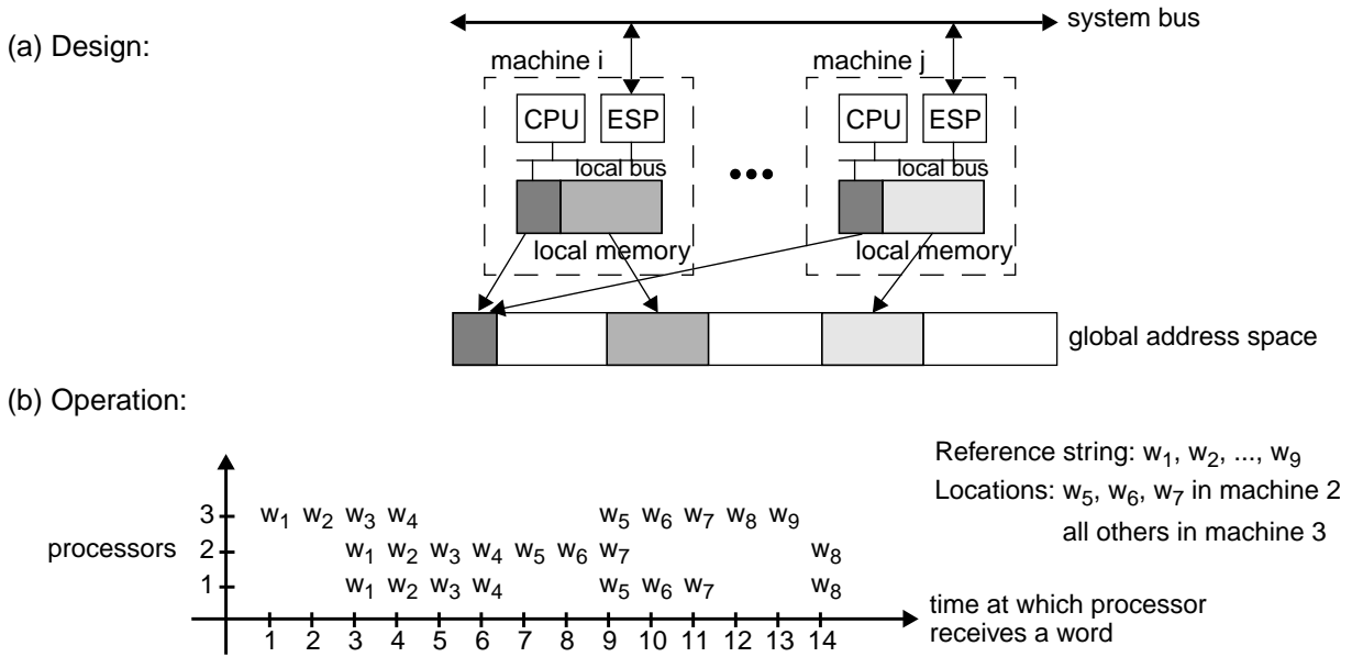
Figure 5. Design and operation of the ESP Massive Memory Machine (taken from [8])
