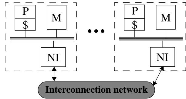
Figure 3. Multicomputer Example
