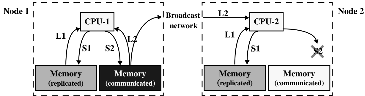
Figure 4. Replicated versus communicated main memory
