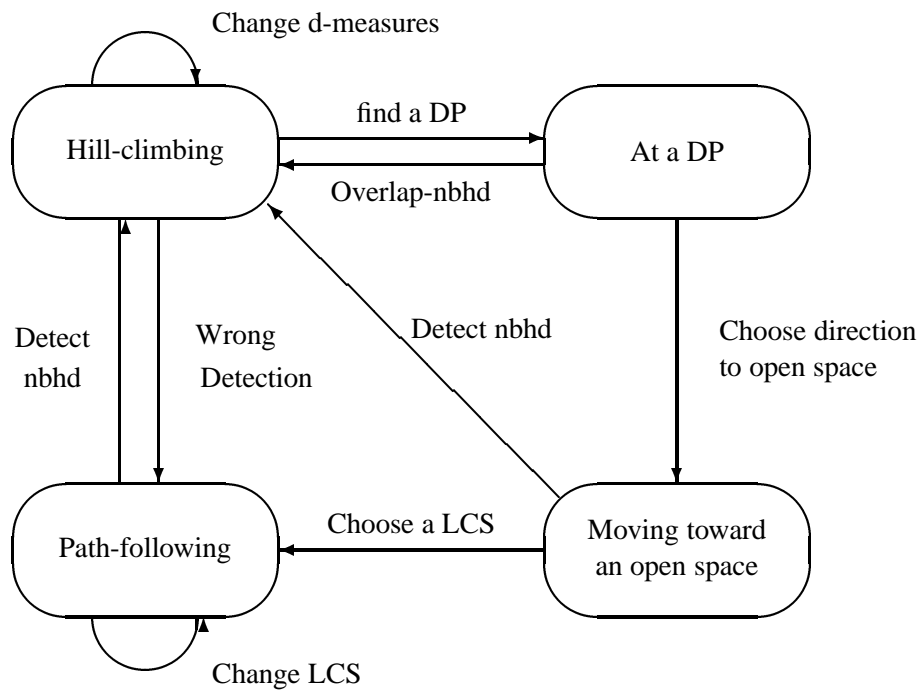
Figure 4: A state-event diagram for the exploration strategy
