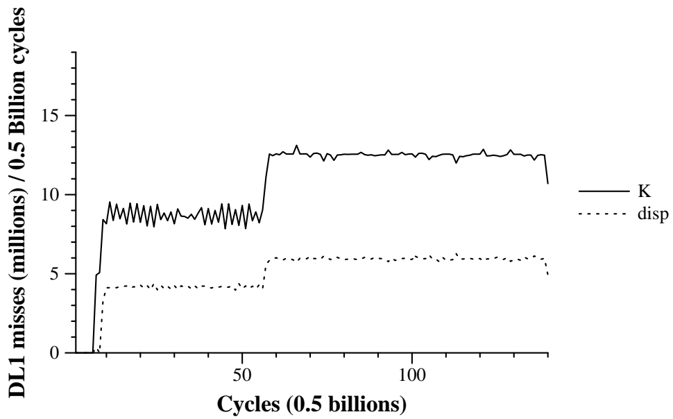
Figure 8: Misses by data structure per 0.5 billion cycles in quake.
