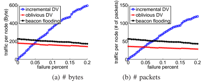
Fig. 6. Control traffic overhead of updating routing state due to topology changes
