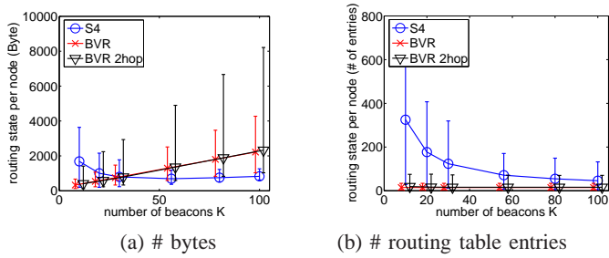
Fig. 4. Routing state comparison: When K = \sqrt{N} , the routing state in S4 is half of routing state in BVR.
