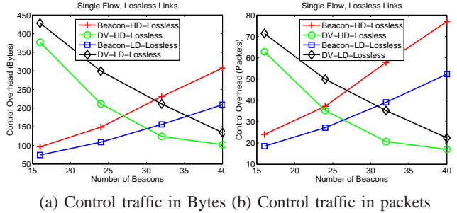
(a) Control traffic in Bytes (b) Control traffic in packets Fig. 12. Control traffic overhead under different numbers of beacons and network densities
