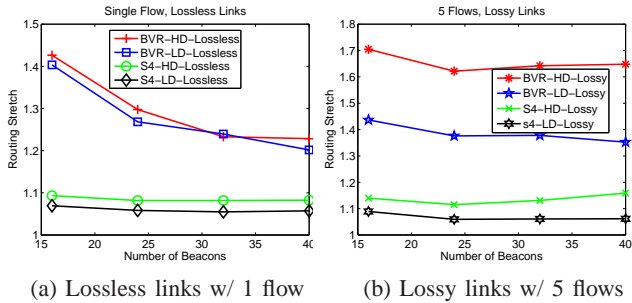
(a) Lossless links w/ 1 flow (b) Lossy links w/ 5 flows Fig. 10. Compare routing stretch under different numbers of beacons, network densities, and traffic patterns.
