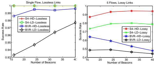
(a) Lossless links w/ 1 flow (b) Lossy links w/ 5 flows Fig. 9. Compare routing success under different numbers of beacons, network densities and traffic patterns.
