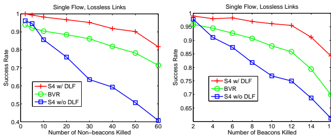
Fig. 17. Impact of DLF on success rate (1000 nodes, 32 beacons, low density)
