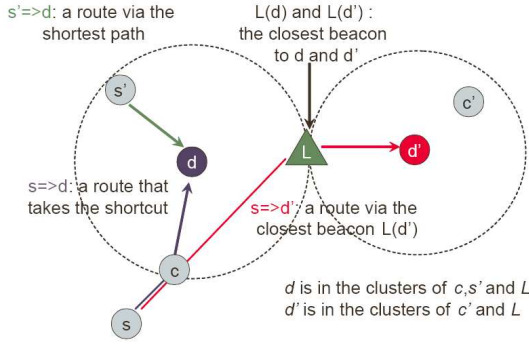
Fig. 1. S4 routing examples. Every node within the circle of d has d in its local cluster. The route s' \rightarrow d is the shortest path; the route s \rightarrow d takes a shortcut at c before reaching L(d) ; the route s \rightarrow d' is through L(d') without shortcut.
