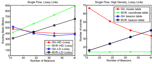
(a) Average routing state (b) number of routing table entries Fig. 13. Routing state comparison under different numbers of beacons and network densities with lossy links (single flow)
