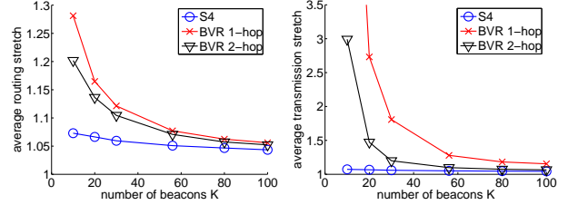
Fig. 3. S4 has routing and transmission stretches close to 1, which is consistently smaller than those of BVR algorithms across all numbers of beacons.
