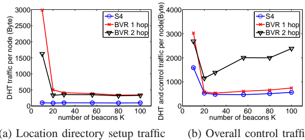
Fig. 7. Control traffic overhead comparison
