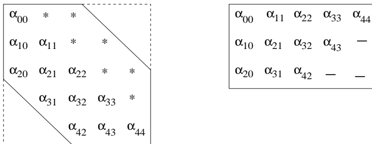
Figure 2: Symmetric 5 \times 5 band matrix with bandwidth k_d = 2 (left) and packed storage used in LAPACK (right). The ‘*’ symbols denote the symmetric entries of the matrix which are not stored in the packed format.
