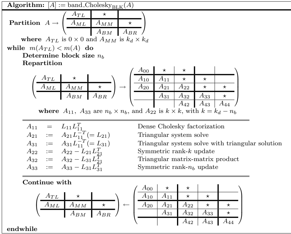
Figure 1: Blocked algorithm for the Cholesky factorization of a band matrix.
