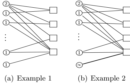
Figure 1: Two example transversal matroids exhibiting the tension between using sampled heavy left-vertices for pricing and over-pricing the right-vertices. The figures are meant only to be illustrative, but can be extended to become counter-examples for certain pricing strategies. In 1(a), we do not want to price all the right-vertices at 2, since we would miss many left-vertices of weight 1. In 1(b), we want to price the bottom right-vertex at 2, since otherwise we would miss the infinite weight left-vertex.
