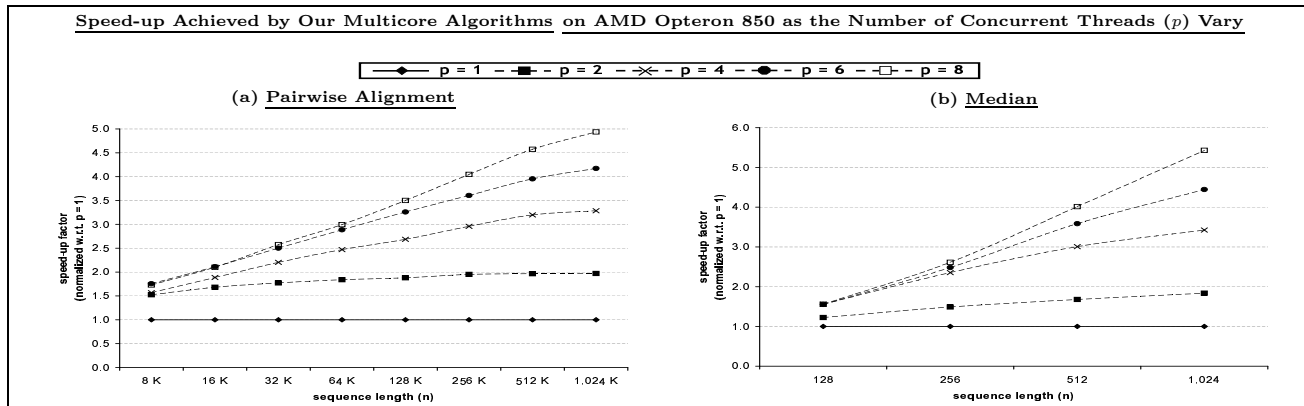
Figure 6: Performance of algorithms for PA and Median on randomly generated sequences over \{A, T, G, C\} .
