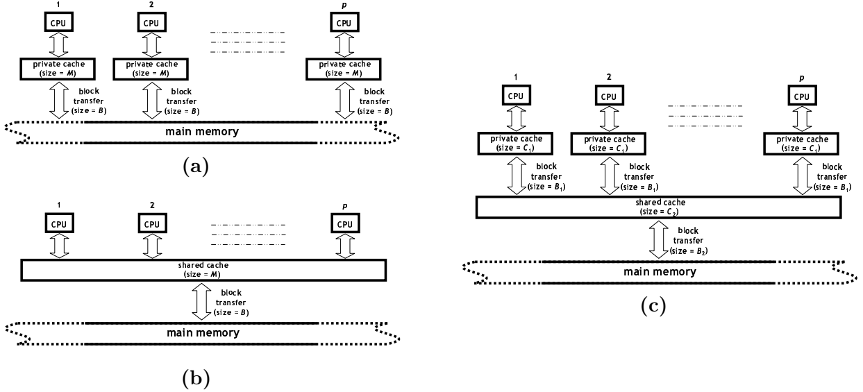
Figure 1: Caching models for CMP: (a) D-CMP , (b) S-CMP , and (c) Multicore .
