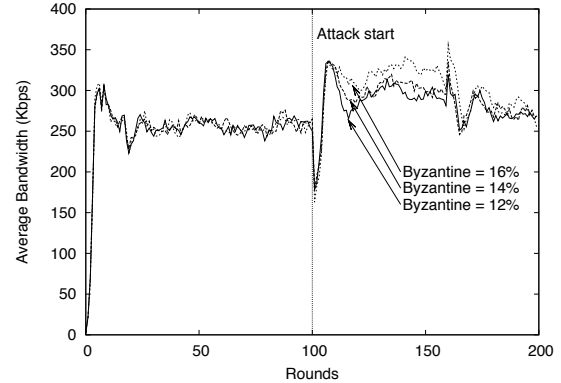
Figure 16: Bandwidth with malicious peers. ( n = 443 )
