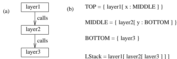
Figure 2.1. Nonpermutable Stacking of Layers
