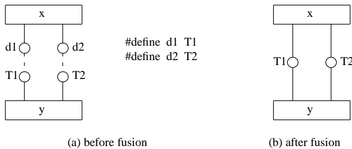
Figure 5.1 Component Fusion via Call Renaming
