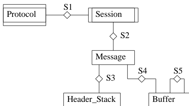
Figure 4.5 The ASYNC Object Model Interface
