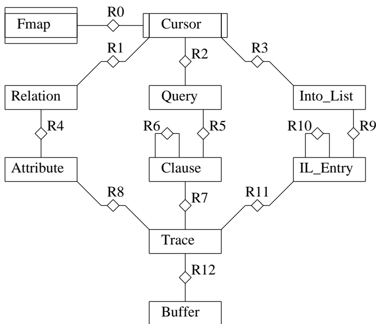
Figure 4.4. The FMAP Object Model Interface
