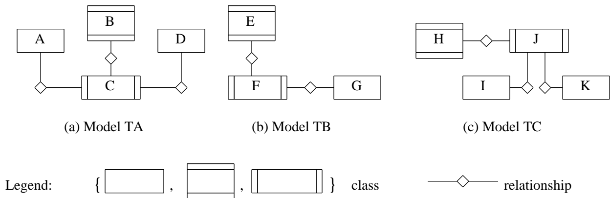
Figure 4.1 Class Diagrams in ER Notation
