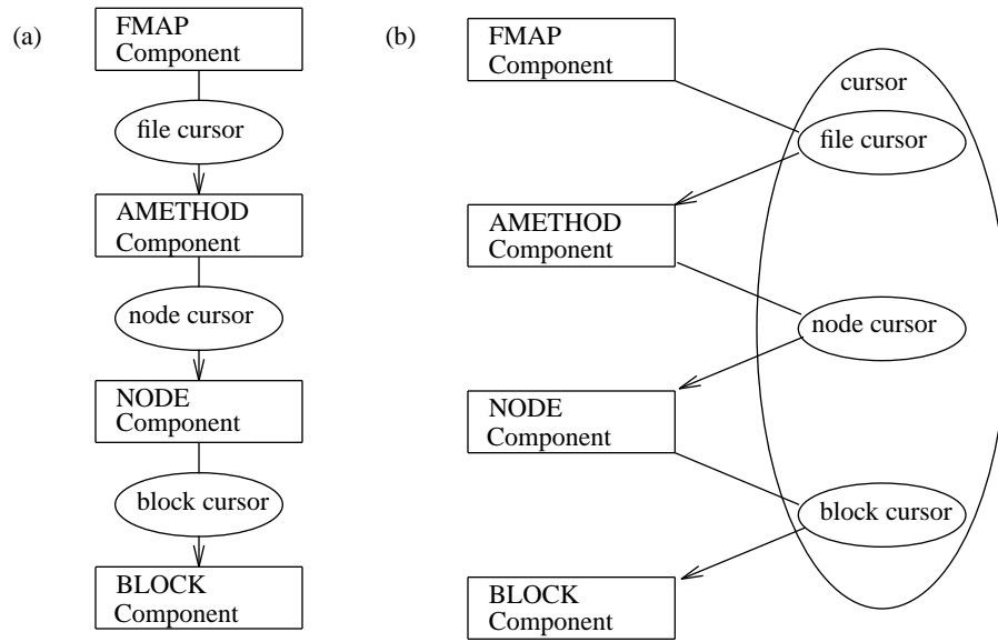
Figure 3.1 Control Block Allocation in Genesis
