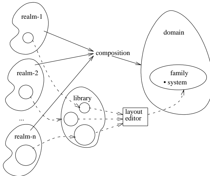
Figure 2.2 Realms, Libraries, Composition, Layout Editor, Family of Systems, and Domain
