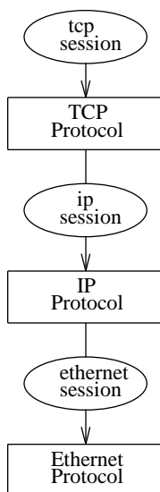
Figure 3.2 Control Block Allocation in Avoca
