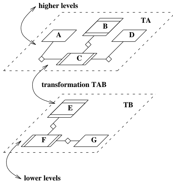
Figure 4.2 Two levels of a Hierarchical System Design
