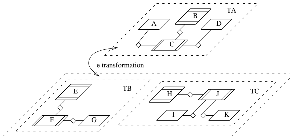
Figure 4.3 Parameterized Component e[ x:TB, y:TC ] : TA
