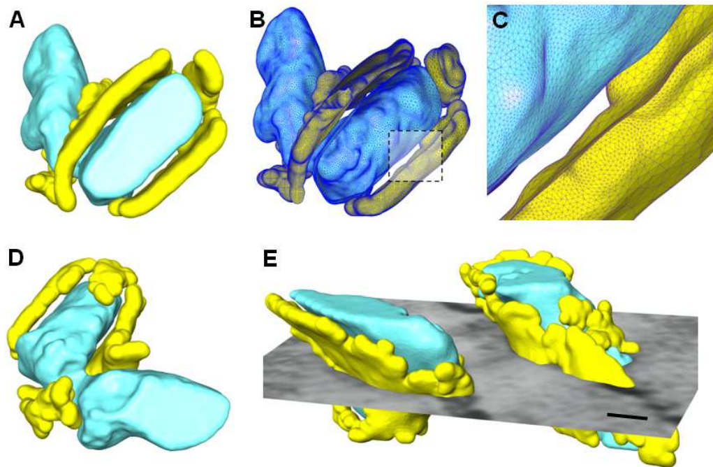
Figure 3: More examples of geometric modeling from EM imaging data. (A) The surfaces rendering of the extracted T-tubules (the thick structures in cyan) surrounded by jSR (the thin structures in yellow). (B) The surface mesh representation with the front part cut out. (C) A close view of the dyadic cleft as indicated by the dashed rectangle in (B). (D) Another view of the same model as shown in (A). (E) Another example of geometric modeling of T-tubules (the thick structures in cyan) and the surrounding jSR (the thin structures in yellow). A cross section of the original image is shown together with the models. Scale bar in (E): 50 nm.
