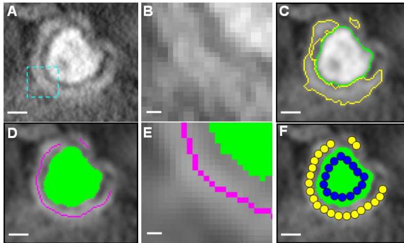
Figure 1: Illustrations of image analysis and geometric modeling. (A) A 3.5nm-thick slice of the electron tomogram of a ventricular cardiomyocyte. This small region, showing a single T-tubule (in the middle) surrounded by junctional sarcoplasmic reticulum (jSR), was taken from a large 3D reconstructed EM map. The size of this sub-volume is 101 \times 91 \times 51 voxels (3.5 nm/voxel). Due to the staining methods specifically used in the current study, T-tubular structures in the EM maps are significantly “darker” than SR and background noise (Note: intensity shown here has been inverted). (B) A close look at the image in the rectangular area indicated in (A). (C) The T-tubule and jSR are segmented using an automatic algorithm. (D) The skeletons of jSR (the curves in magenta) are automatically extracted based on the segmented jSR from (C). (E) A close look at the skeletons and boundaries in the same area indicated in (A). (F) Schematic illustration of the sphere-packing method to create pseudo-molecules of T-tubules and jSR. Scale bars: 50 nm in (A,C,D,F) and 10 nm in (B,E).
