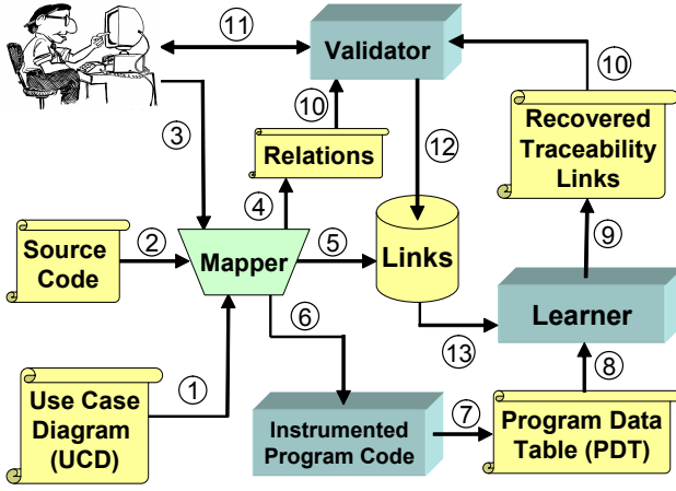
Figure 3: LeanART architecture.
