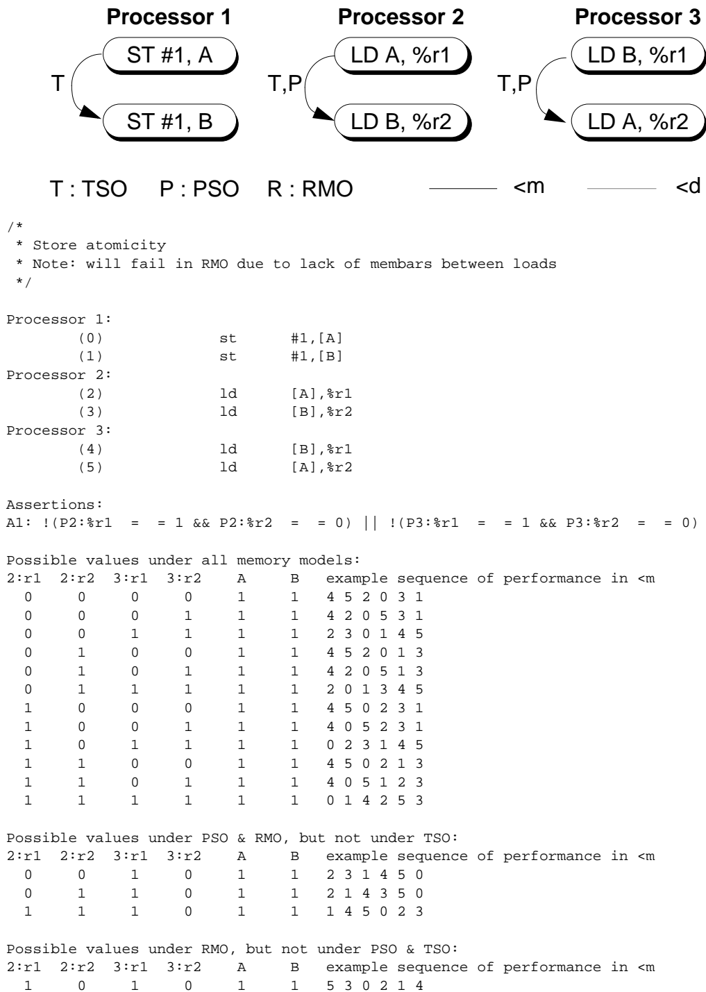
Figure 44—Store Atomicity Example
