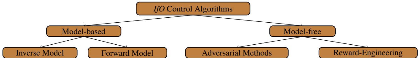
Figure 1: A diagrammatic representation of categorization of the I/O control algorithm. The algorithms can be categorized into two groups: (1) model-based algorithms in which the algorithms may use either a forward dynamics model [Edwards et al. , 2019] or an inverse dynamics model [Torabi et al. , 2018; Nair et al. , 2017]. (2) Model-free algorithms, which itself can be categorized to adversarial methods [Torabi et al. , 2019c; Merel et al. , 2017; Stadie et al. , 2017] and reward engineering [Sermanet et al. , 2018; Gupta et al. , 2018; Liu et al. , 2018].
