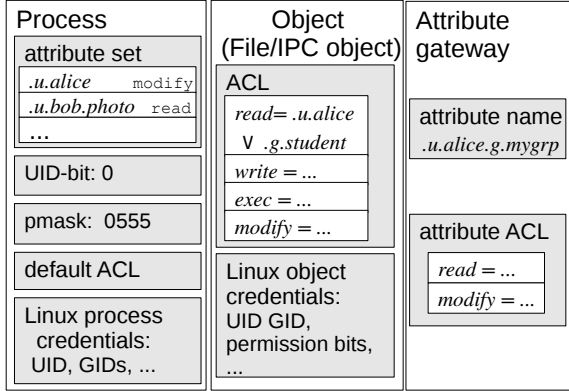
Figure 1: Overview of processes, objects and attribute gateways in DCAC.
