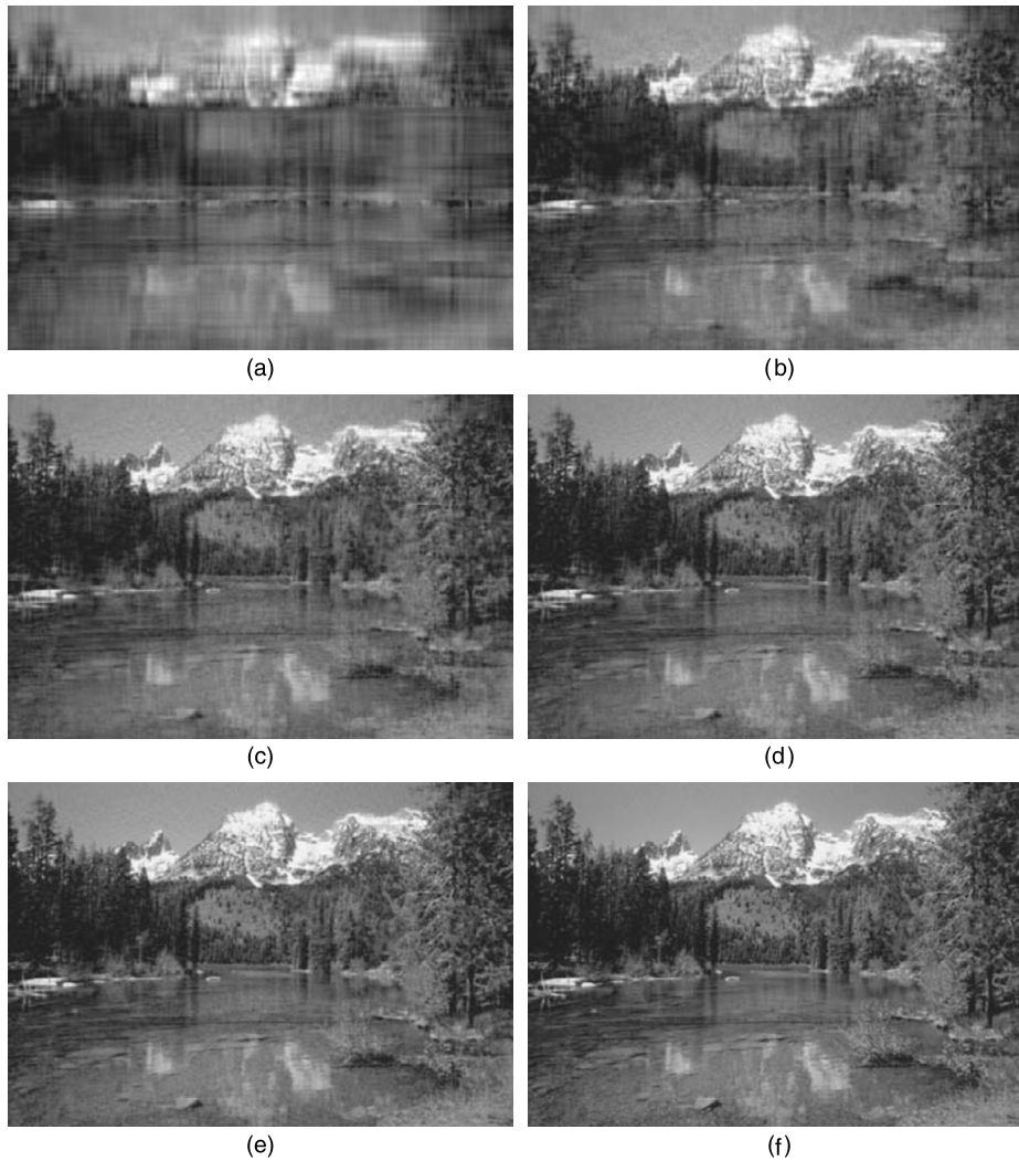
FIGURE 9.3 Compressed images of “Grand Teton”: (a) using 10 terms; (b) using 25 terms; (c) using 50 terms; (d) using 75 terms; (e) using 100 terms; (f) using 200 terms
