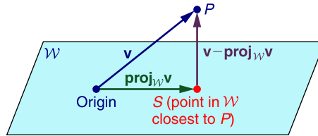
FIGURE 6.5 The minimum distance from P to \mathcal{W} , \|\mathbf{v} - \text{proj}_{\mathcal{W}} \mathbf{v}\|
