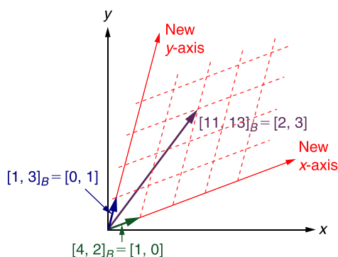
FIGURE 4.6 A B -coordinate grid in \mathbb{R}^2 : picturing [11, 13] in B -coordinates
