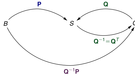
FIGURE 6.1 Visualizing Q^{-1}P as the transition matrix from B to C
