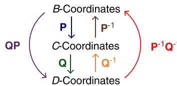
FIGURE 4.8 Transition matrices used to convert between B -, C -, and D -coordinates in \mathcal{P}_2
