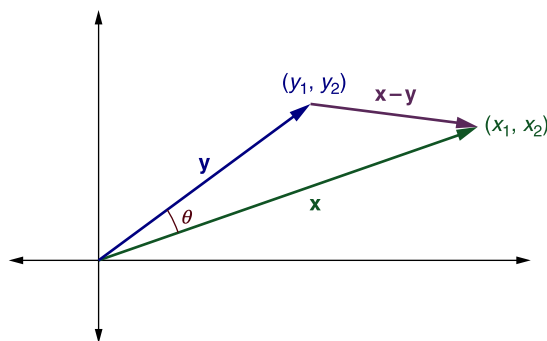
FIGURE 1.15 The angle \theta between two nonzero vectors \mathbf{x} and \mathbf{y} in \mathbb{R}^2
