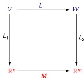
FIGURE 5.12 The linear transformations L and M and the isomorphisms L_1 and L_2 in Theorem 5.21
