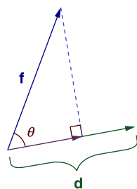
FIGURE 1.20 Projection \|\mathbf{f}\| \cos \theta of a vector force \mathbf{f} onto a vector displacement \mathbf{d} , with angle \theta between \mathbf{f} and \mathbf{d}
