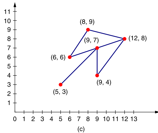
FIGURE 8.27 (a) Figure for Exercise 4; (b) figure for Exercise 5; (c) figure for Exercise 6
