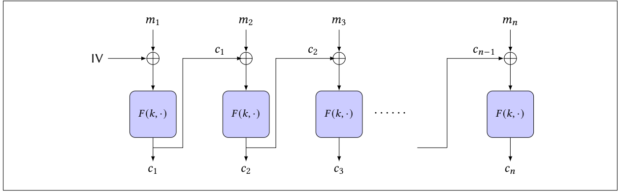
Figure 3: CBC encryption
