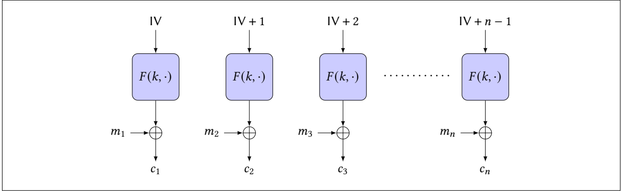
Figure 1: Counter-mode encryption
