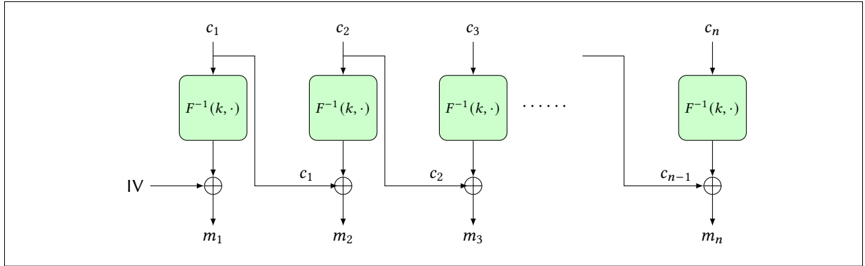
Figure 4: CBC decryption
