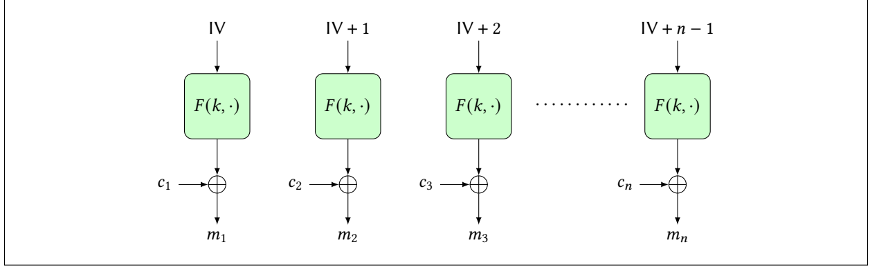
Figure 2: Counter-mode decryption
