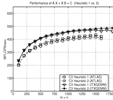
Fig. 10. Performance of the triangular Sylvester equation solvers using Heuristic 1 and Heuristic 2.
