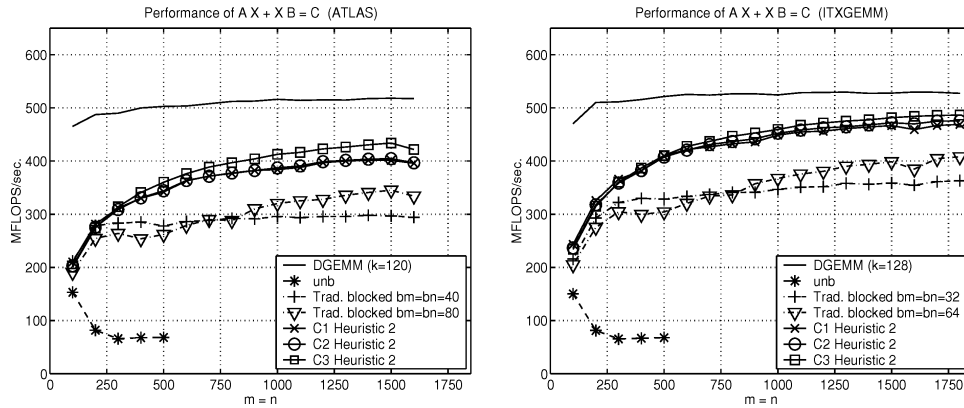
Fig. 9. Performance of our triangular Sylvester equation solvers using DGEMM from ATLAS R3.2 (Left) and ITXGEMM (Right).
