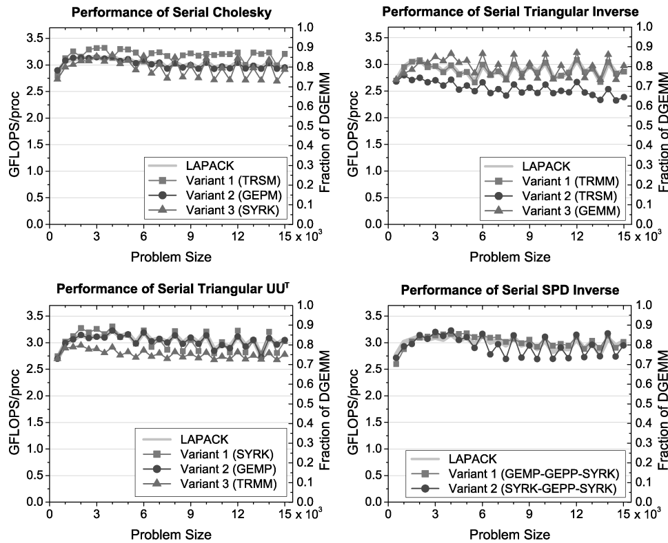
Fig. 10. Sequential performance on the IBM Power4 system.
