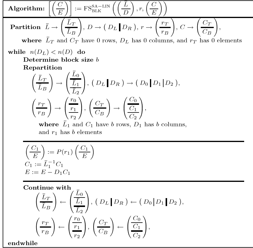
Fig. 5. SA-LINPACK blocked algorithm for the update of (C^T, E^T)^T , consistent with the SA-LINPACK blocked LU factorization of (U^T, D^T)^T .
