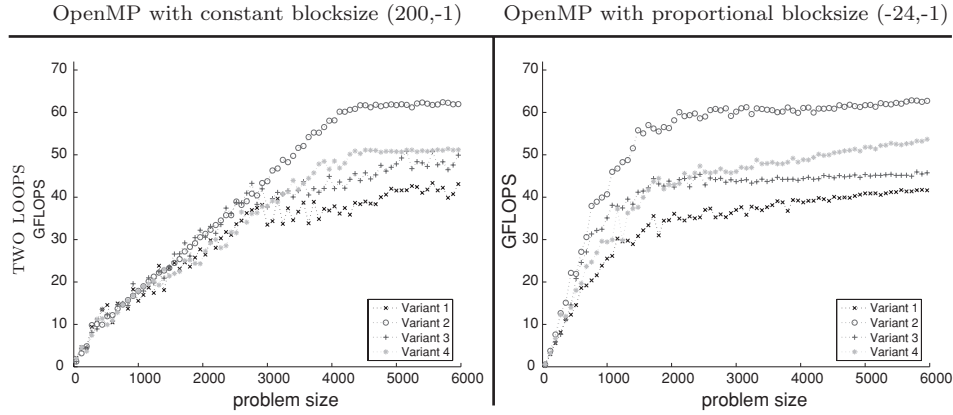
Fig. 13. Performance of OpenMP task queue parallelizations (12 threads) of SYRK Variants 1 through 4 where m equals the problem size and k = 200 . The experiments on the left were performed with a constant blocksize of 200 while those on the right were performed with a proportional blocksize that partitioned the matrix equally through 24 iterations. Only results for the two-loop task partitioning option are shown. Bottom line: Proportional blocking enables superior load balancing for small to medium-sized problems, allowing performance to ramp up quickly. Variant 2 outperforms all other variants due to a combination of enqueueing variable-sized tasks in descending order of cost and properties inherent in the dgemm implementation used to compute the matrix products associated with these tasks.
