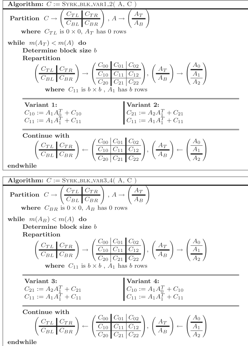
Fig. 3. Blocked algorithms for computing C := AA^T + C . The top algorithm implements Variants 1 and 2, corresponding to Loop-Invariants 1 and 2 in Figure 2. The bottom algorithm implements Variants 3 and 4, corresponding to Loop-Invariants 3 and 4 in Figure 2. Variants 1 and 2 share the same loop-body updates as Variants 4 and 3, respectively. Variants 1 and 2 sweep through C from the top-left to the bottom-right, and A from top to bottom, while Variants 3 and 4 traverse the matrices in the opposite directions.
