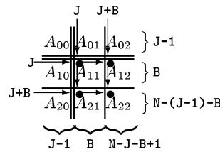
Fig. 4. Partitioning of matrix A with all dimensions annotated when A_{00} = A_{TL} is (j-1) \times (j-1) .
