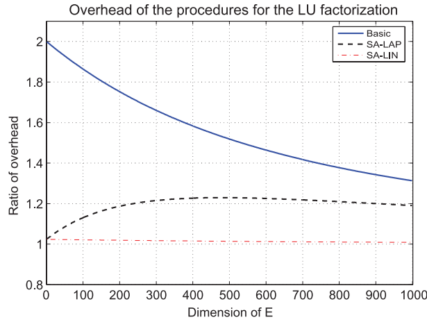
Fig. 6. Overhead cost of the different approaches to compute the LU factorization in Eq. (1) with respect to the cost of the LU factorization with partial pivoting.
