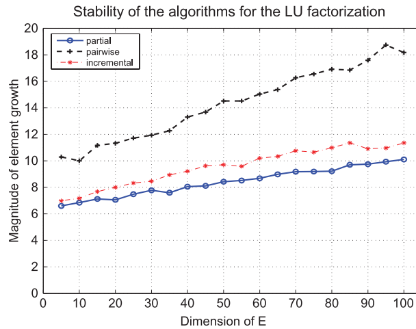
Fig. 7. Element growth in LU factorization using different pivoting techniques.
