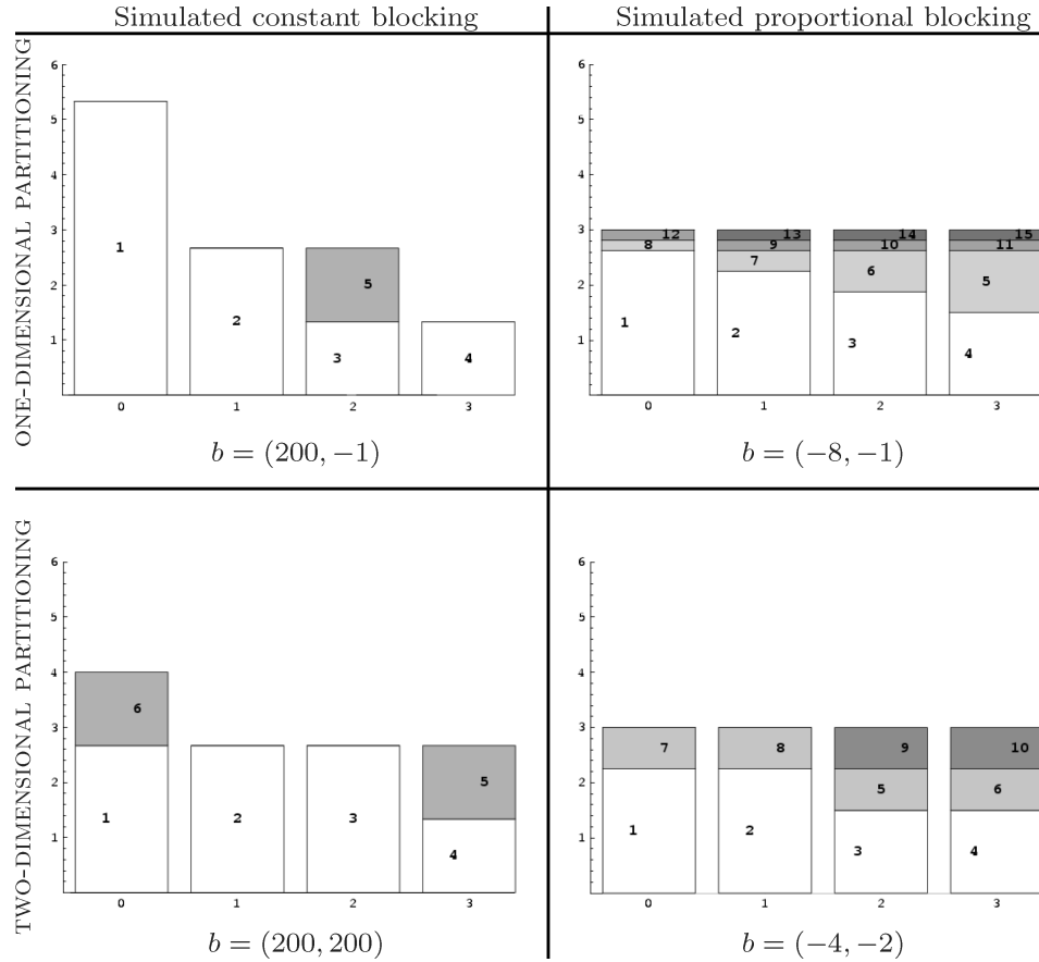
Fig. 12. Simulated scheduling of tasks to four threads for Variant 2 when m = 600 and k = 200 for various blocksize and partitioning schemes. The axes' units are similar to those of Figures 7 and 10. Bottom line: Depending on the problem size, tasks created with constant blocking sometimes fail to distribute well among threads. Moving to a constant 2D partitioning helps, but remains suboptimal. In contrast, both 1D and 2D proportional blocking create the opportunity for ideal load-balance regardless of problem size.
