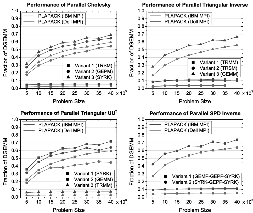
Fig. 12. Parallel performance for PLAPACK-based implementations (C interfaced with MPI).
