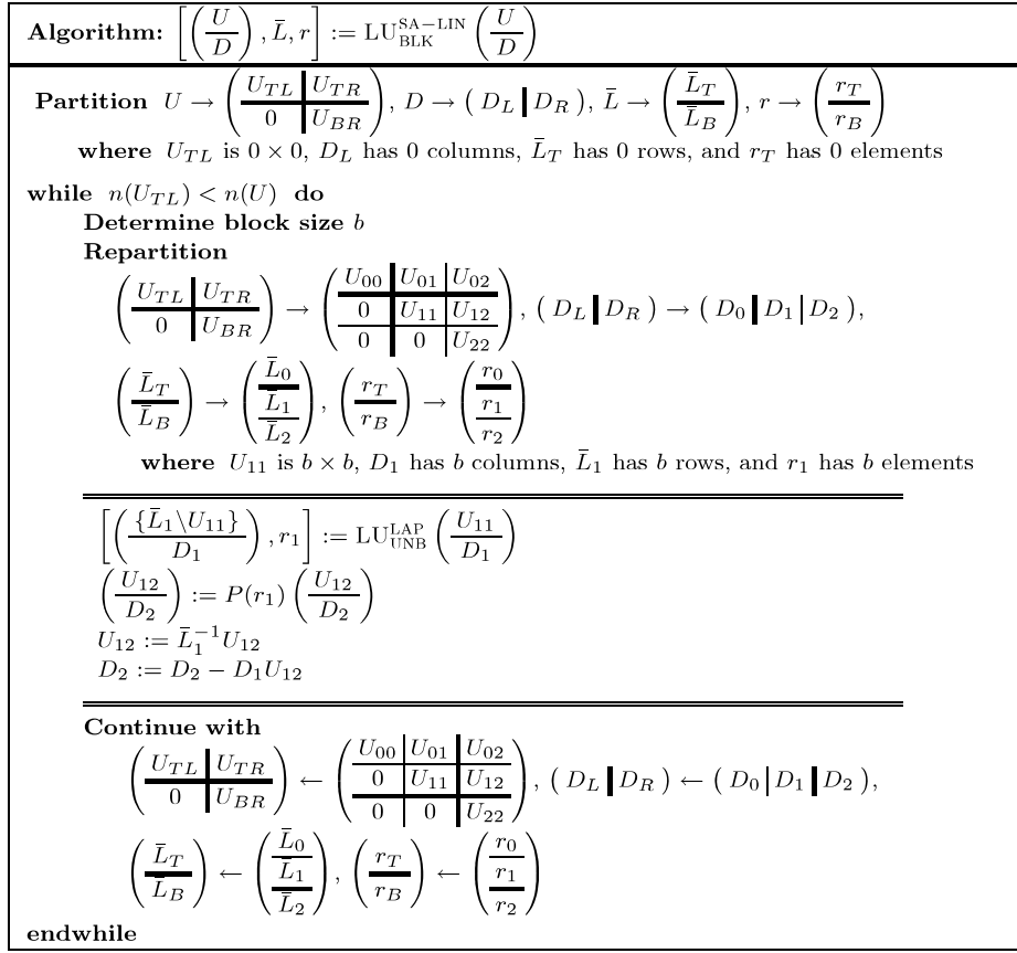
Fig. 3. SA-LINPACK blocked algorithm for the LU factorization of (U^T, D^T)^T built upon an LAPACK blocked factorization.
