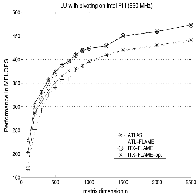
Fig. 11. Performance of LU factorization with pivoting followed by forward and backward substitution.
