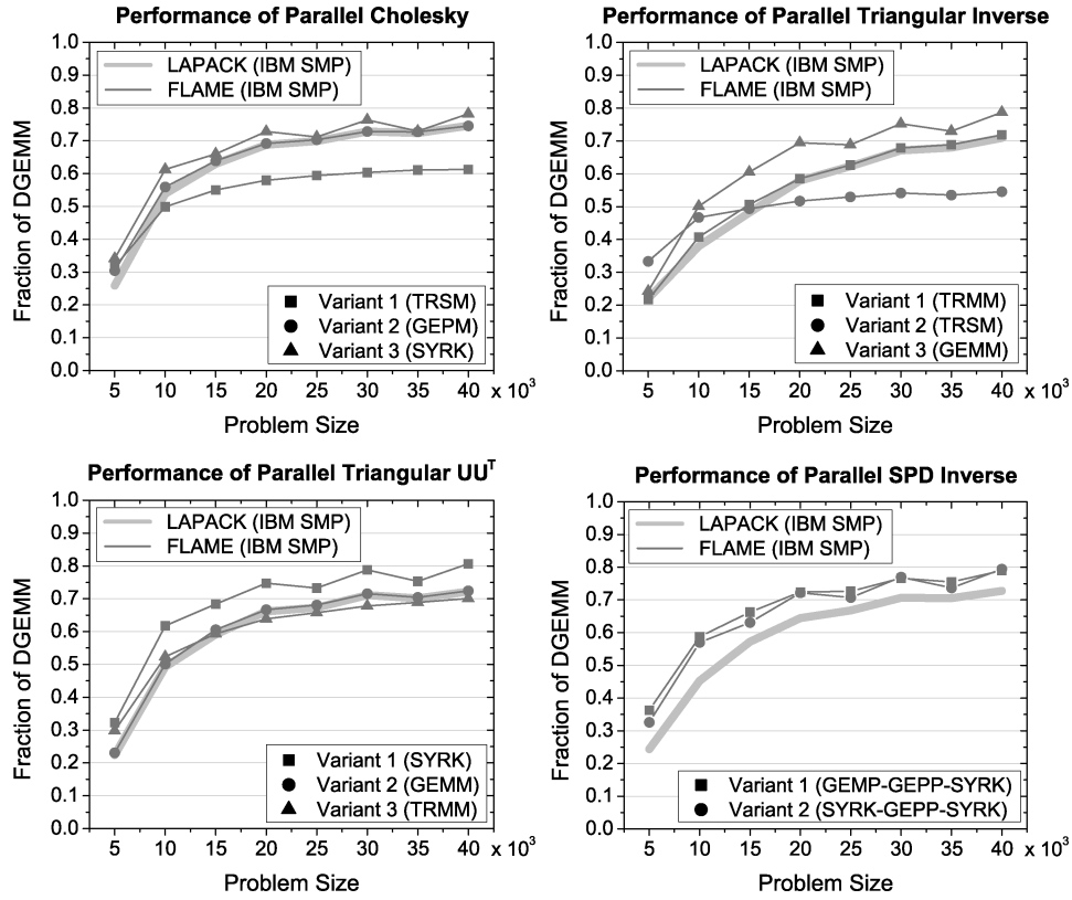
Fig. 11. Parallel performance on the 16 CPU IBM Power 4 SMP system.
