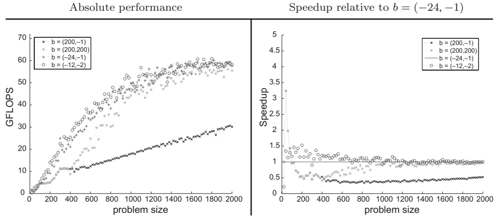
Fig. 16. Performance of FLAME workqueueing parallelization (12 threads) of SYRK Variant 2 when m equals the problem size and k = 200 . The problem size range and increments have been reduced from Figure 13 to show more detail for small problems. Bottom line: A proportional 2D partitioning performs noticeably better for certain smaller problems and on par with a proportional 1D partitioning for larger problems.
