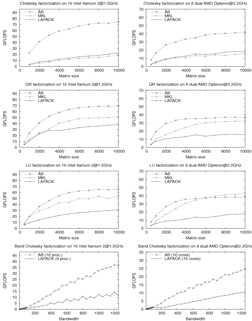
Fig. 10. Performance of the multithreaded factorization algorithms.
