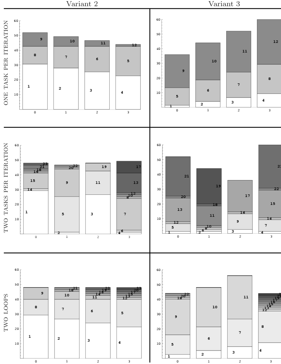
Fig. 7. Simulated OpenMP task queues scheduling of tasks to four threads for Variants 2 and 3 when m = 2400 , k = 200 , and the blocksize equals 200. The sum of the heights of the rectangles in each x-axis column correspond to the total amount of work assigned to each thread. The y-axis is in units of FLOPs \times 10^6 (millions of FLOPs). Load balance is ideal when all threads receive equal work. Bottom line: Load balance is determined by the number of tasks created, the cost of each task, and the order in which tasks are enqueued.
