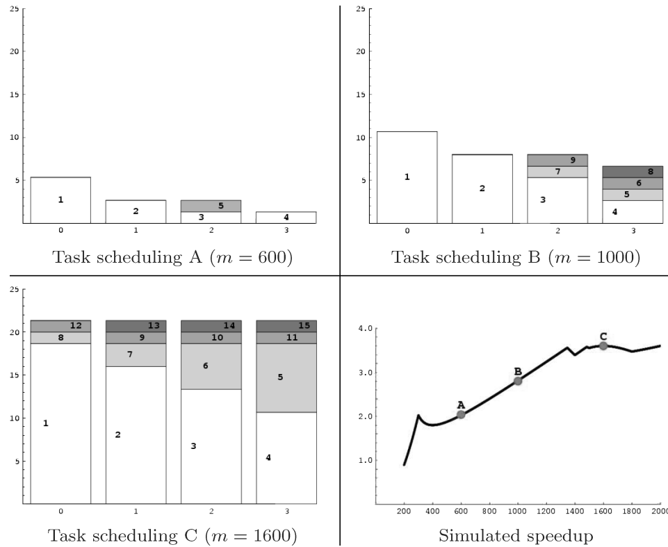
Fig. 10. Simulated OpenMP task queues scheduling of tasks to four threads for Variant 2 shown for select values of m when k = 200 . The two-loop parallelization for Variant 2 was used, which enqueues tasks in sorted order. Also, the blocksize used was 200. The axes' units of the three task scheduling graphs is similar to that of Figure 7. The corresponding speedup of each task scheduling is marked on the curve shown in the lower-right graph, in which we assume dgemm and dsyrk consistently perform at 90% of peak efficiency. Bottom line: Given a one-dimensional constant blocking, some threads fall idle before others due to poor distribution of work, where the largest variable-sized GEMM tasks become bottlenecks. This load-imbalance hinders parallel speedup and thus results in limited performance for many smaller problem sizes.
