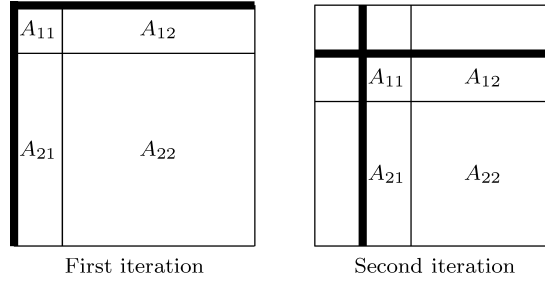
Fig. 3. First two iterations of the blocked algorithm in Figure 1 (right).
