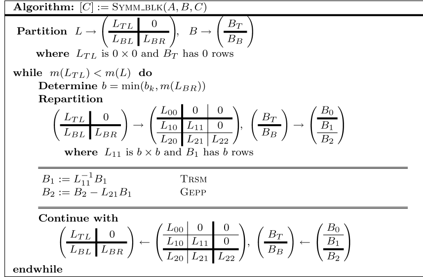
Fig. 10. Algorithm for computing TRSM that casts most computation in terms of GEPP.
