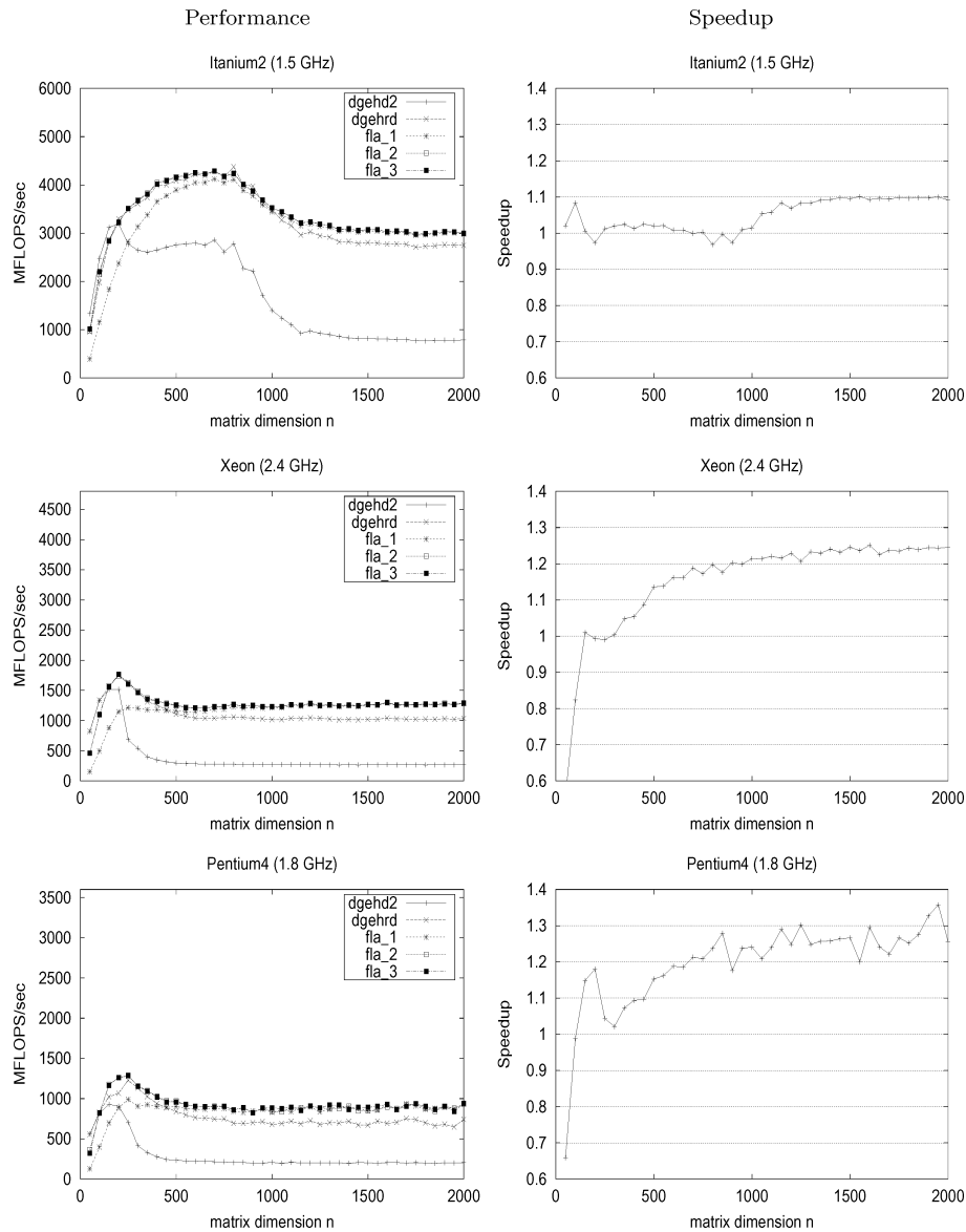
Fig. 5. Performance on various architectures as a function of matrix size, n , using a block size of nb = 32 . When the matrix-vector product operation is relatively fast (on the Itanium 2), the overall performance is better and the speedup that is observed is less, since less time is spent in matrix-vector product. When the matrix-vector product is slow (on the Xeon and Pentium 4), the overall performance is worse, and the speedup gained by shifting computation from the matrix-vector product to the matrix-matrix product is more noticeable.
