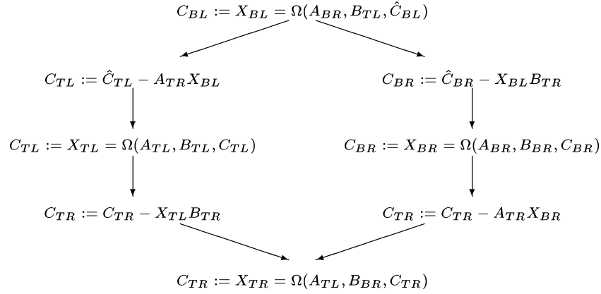
Fig. 7. Data dependencies for the partitioned triangular Sylvester matrix equation.
