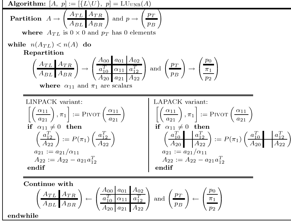
Fig. 1. LINPACK and LAPACK unblocked algorithms for the LU factorization.
