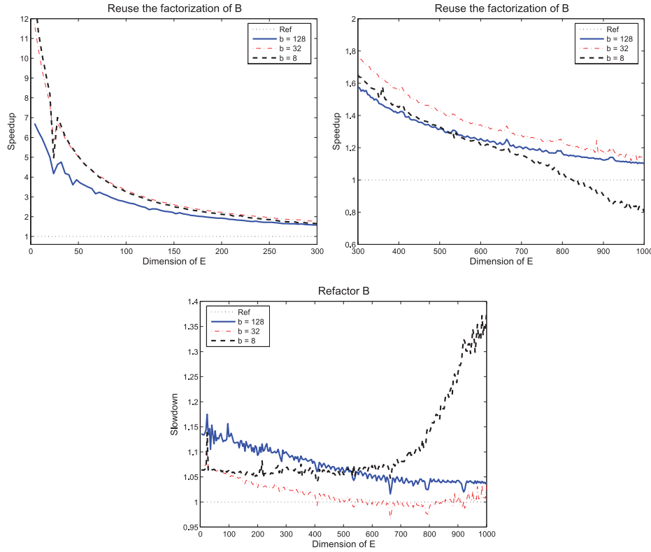
Fig. 8. Top: speedup attained when B is not refactored, over LU factorization with partial pivoting of the entire matrix; bottom: slowdown for the first factorization (when B must also be factored).
