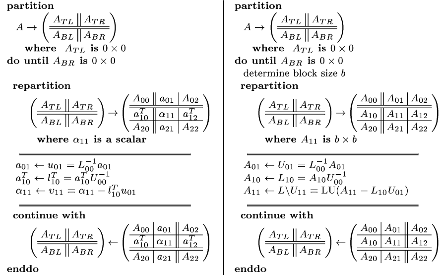
Fig. 2. Unblocked and blocked versions of the lazy variant for computing the LU factorization of a square matrix A (without pivoting).
