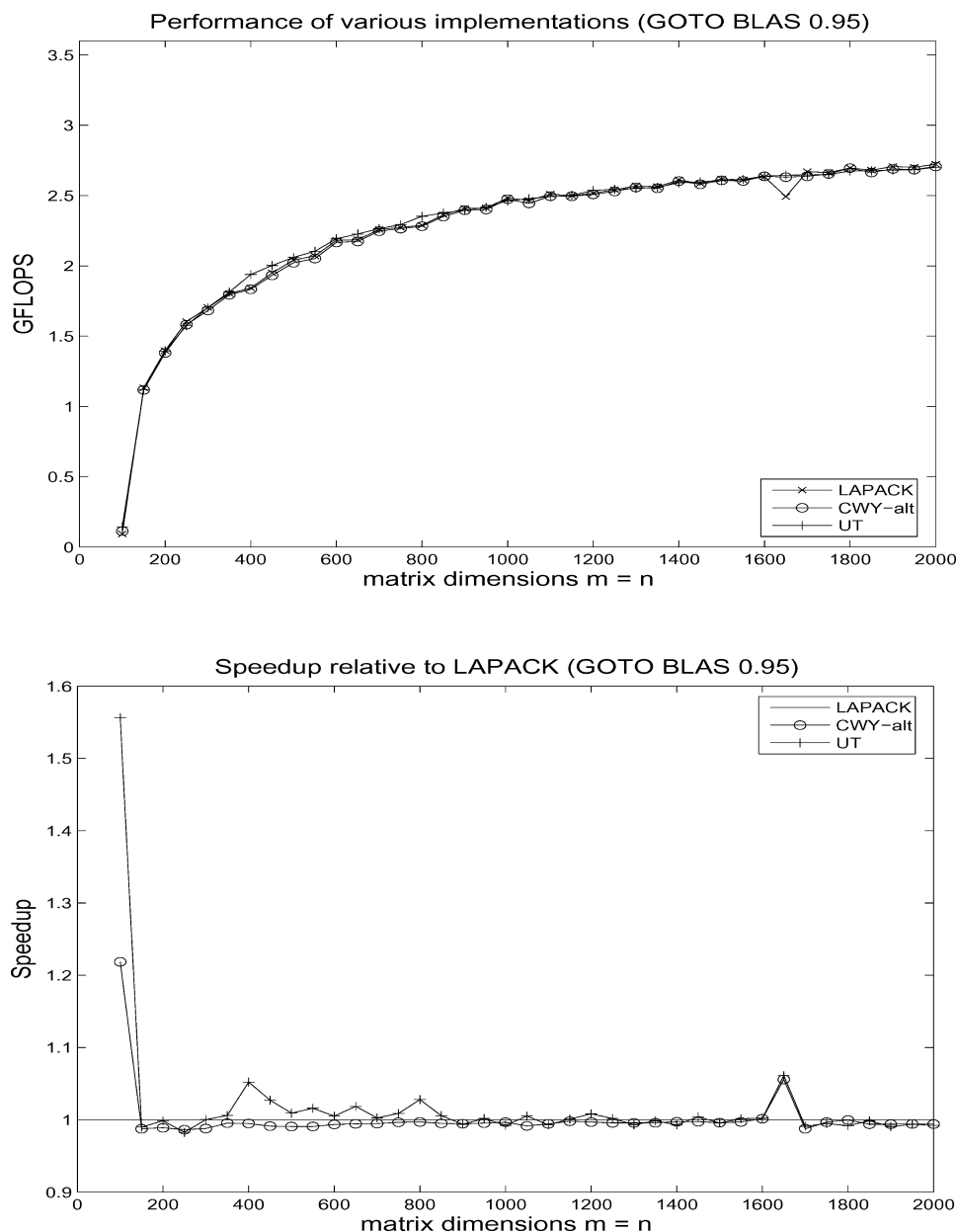
Fig. 4. Performance of the various implementations on an Intel Itanium 2 (900MHz) server (single CPU), linked to GOTO BLAS release 0.95.
