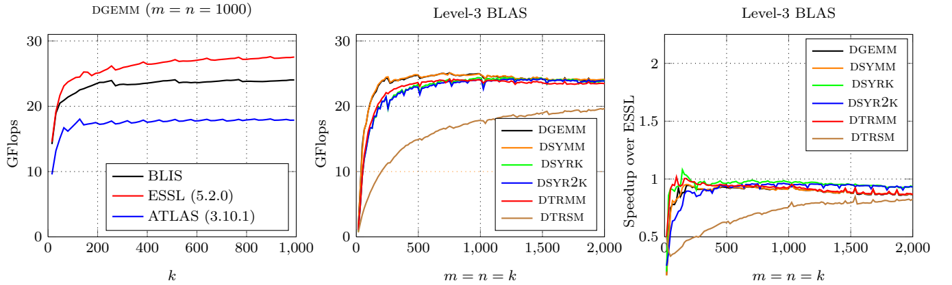
Figure 6: Performance on the IBM IBM Power7 processor (one core).
