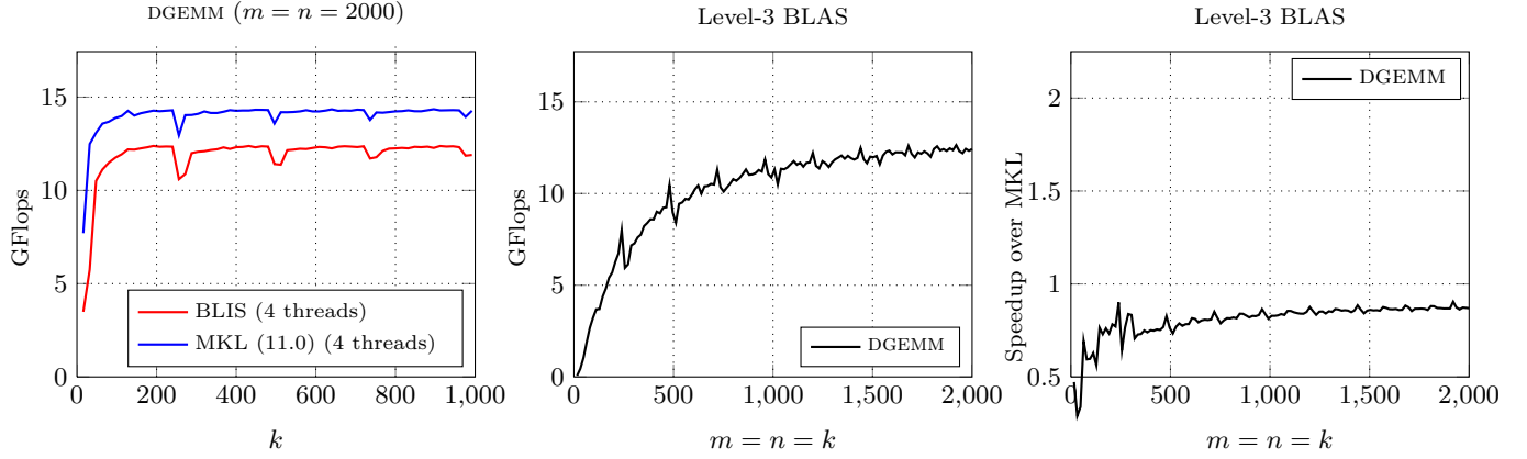
Figure 9: Performance on the Intel Xeon Phi (MIC) processor (one core). A single thread can only issue one instruction every other cycle so that hyperthreading with up to four threads is required.
