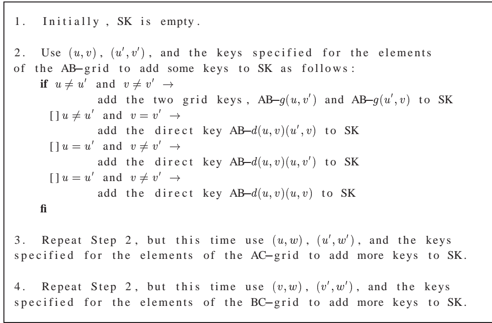
Fig. 2. Algorithm 2 for Selecting Keys
