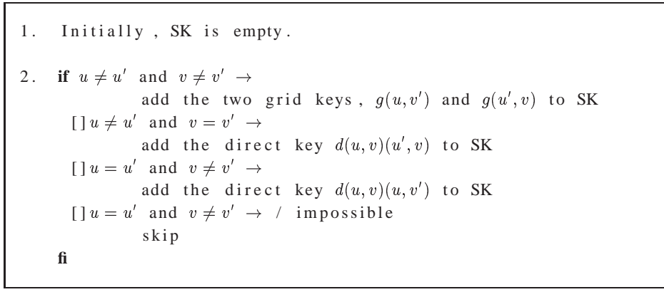
Fig. 1. Algorithm 1 for Selecting Keys
