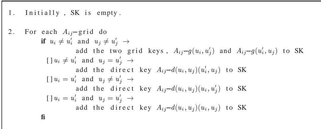
Fig. 3. Algorithm 3 for Selecting Keys
