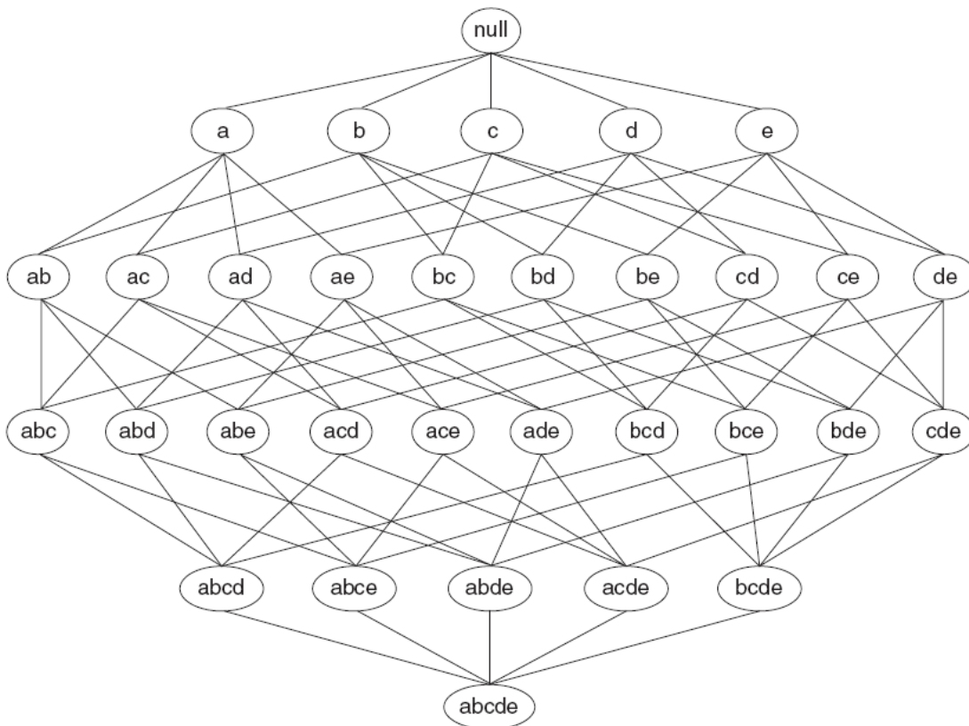
Figure 6.33. An itemset lattice
