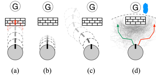
Figure 2: (a) Unsafe trajectory leading to a collision. (b) Safe but sub-optimal trajectory. (c) Optimal and safe trajectory. (d) An instance of the planning phase.
