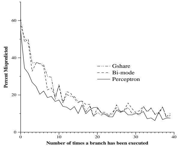
Figure 6: Average Training Times for gcc. The x axis is the number of times a branch has been executed. The y axis is the average, over all branches in the program, of 1 if the branch was mispredicted, 0 otherwise. Over time, this statistic tracks how quickly each predictor learns. The perceptron predictor achieves greater accuracy earlier than the other two methods.
