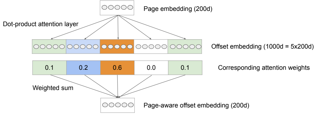
Figure 3: Conditional attention embedding.
