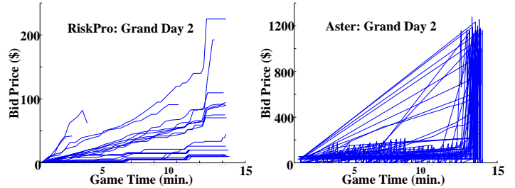
Figure 2: Graphs of two different agents’ bidding patterns over many games. Each line represents one game’s worth of bidding in a single auction. Left: RiskPro never bids over $250 in the games plotted. Right: Aster consistently bids over $1000 for rooms (note the different scales).
