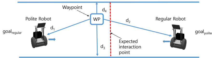
Figure 2: The four features that represent the waypoint. d_1, d_2 represent the distance from the waypoint to each robot. d_3, d_4 represent the distance between the waypoint and the closest obstacle on each side perpendicular to the line connecting the two robots.
