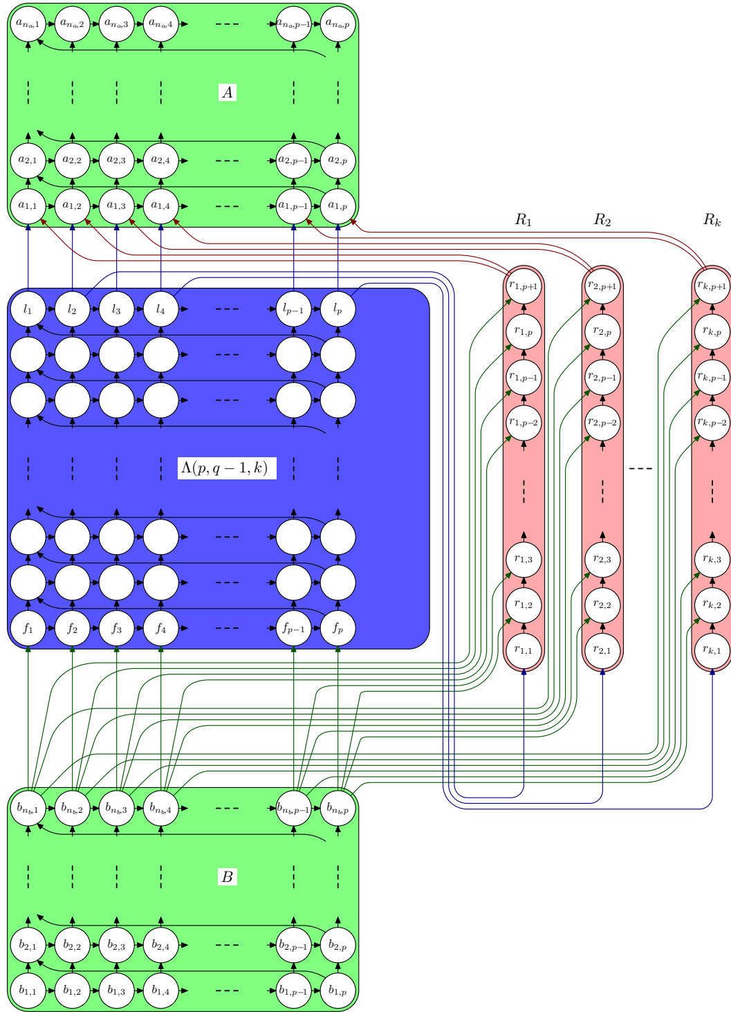
Fig. 8. Building block N(p, q, k) in graph separating black and black-white pebbling (here k = p/2 ).
