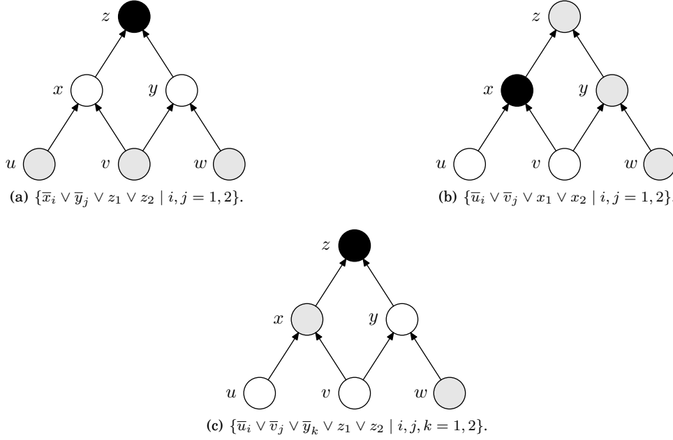
Fig. 2. Black and white pebbles and (intuitively) corresponding sets of clauses.
