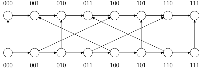
Fig. 6. Bit reversal graph \Delta(8, \text{rev}) on 8 elements.
