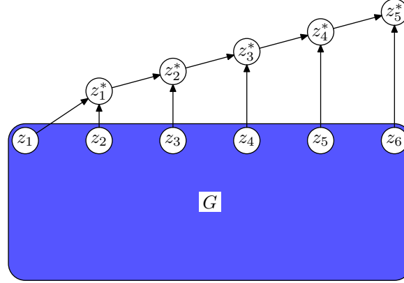
Fig. 5. Schematic illustration of single-sink version \hat{G} of graph G .
