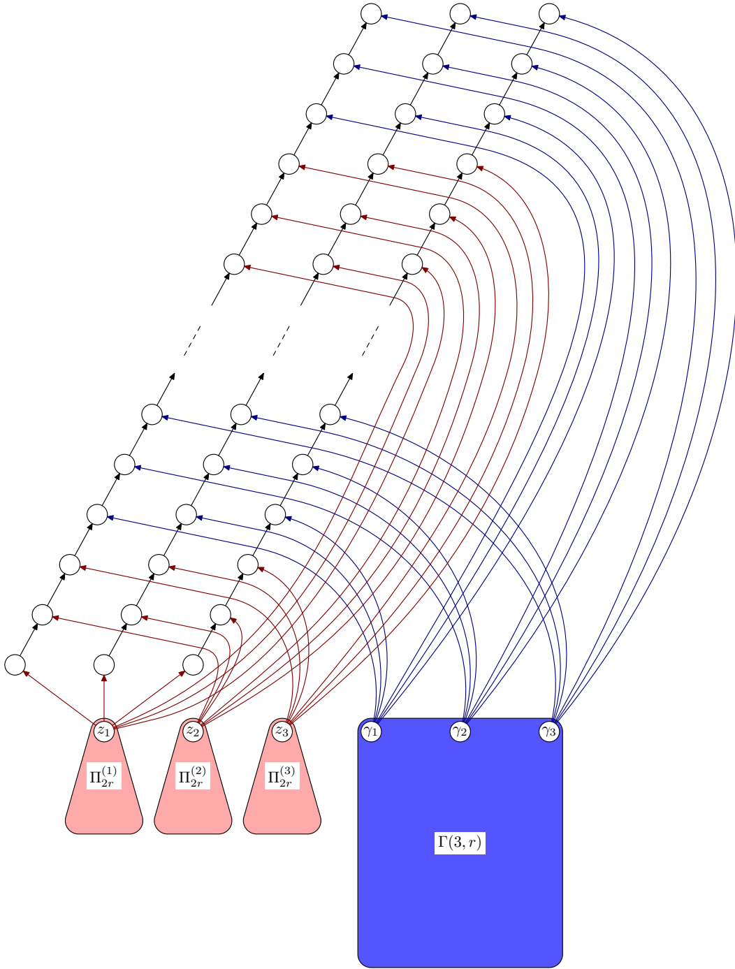
Fig. 4. Inductive definition of Carlson-Savage graph \Gamma(3, r+1) with 3 spines and sinks.
