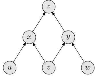
(a) Pyramid graph \Pi_2 of height 2.
