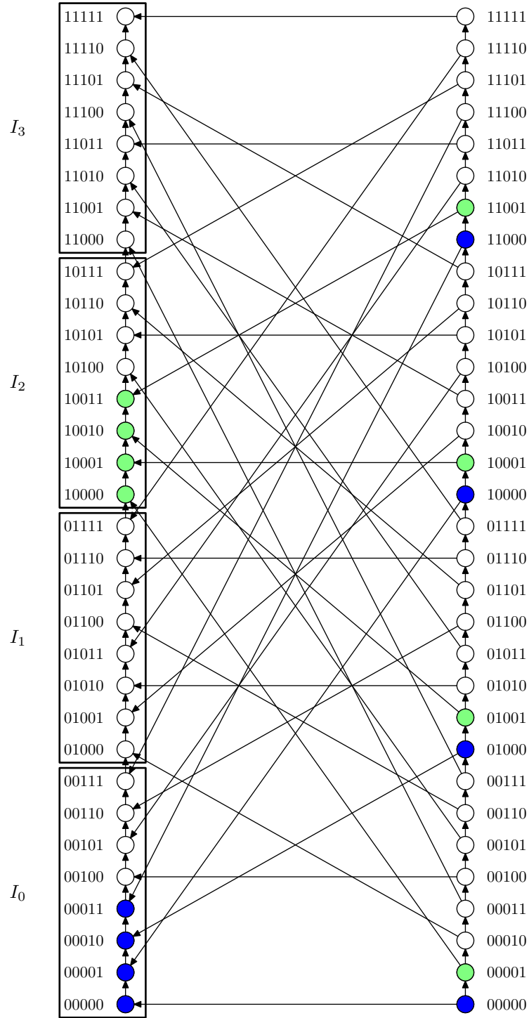
Fig. 7. Intervals I_j for r = 2 in \Delta(32, \text{rev}) and 0th chunks in I_0 and I_{\text{rev}_r(1)} = I_2 with inverse images.
