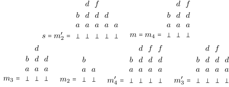
Fig. 3. Illustration for the construction in the second step of the proof of Lemma 5.25.
