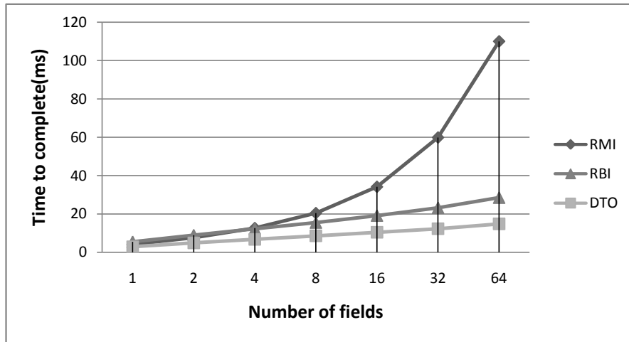
Fig. 7: Performance Comparison between RMI, RBI, and DTO versions
