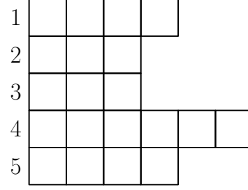
(b) The histogram of \mathbf{w} (on its side).
