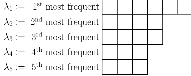
(c) The sorted histogram of \mathbf{w} .
