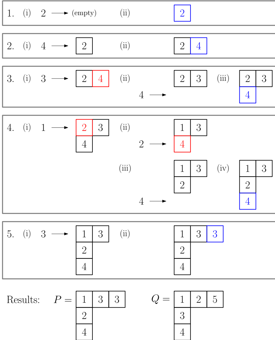
Figure 3.1: The construction of the insertion tableau P from the RSK algorithm applied to the word w = 24313 . Each large gray box corresponds to a Schensted insertion, each red box corresponds to a bumped letter, and each blue box corresponds to a newly created cell.
